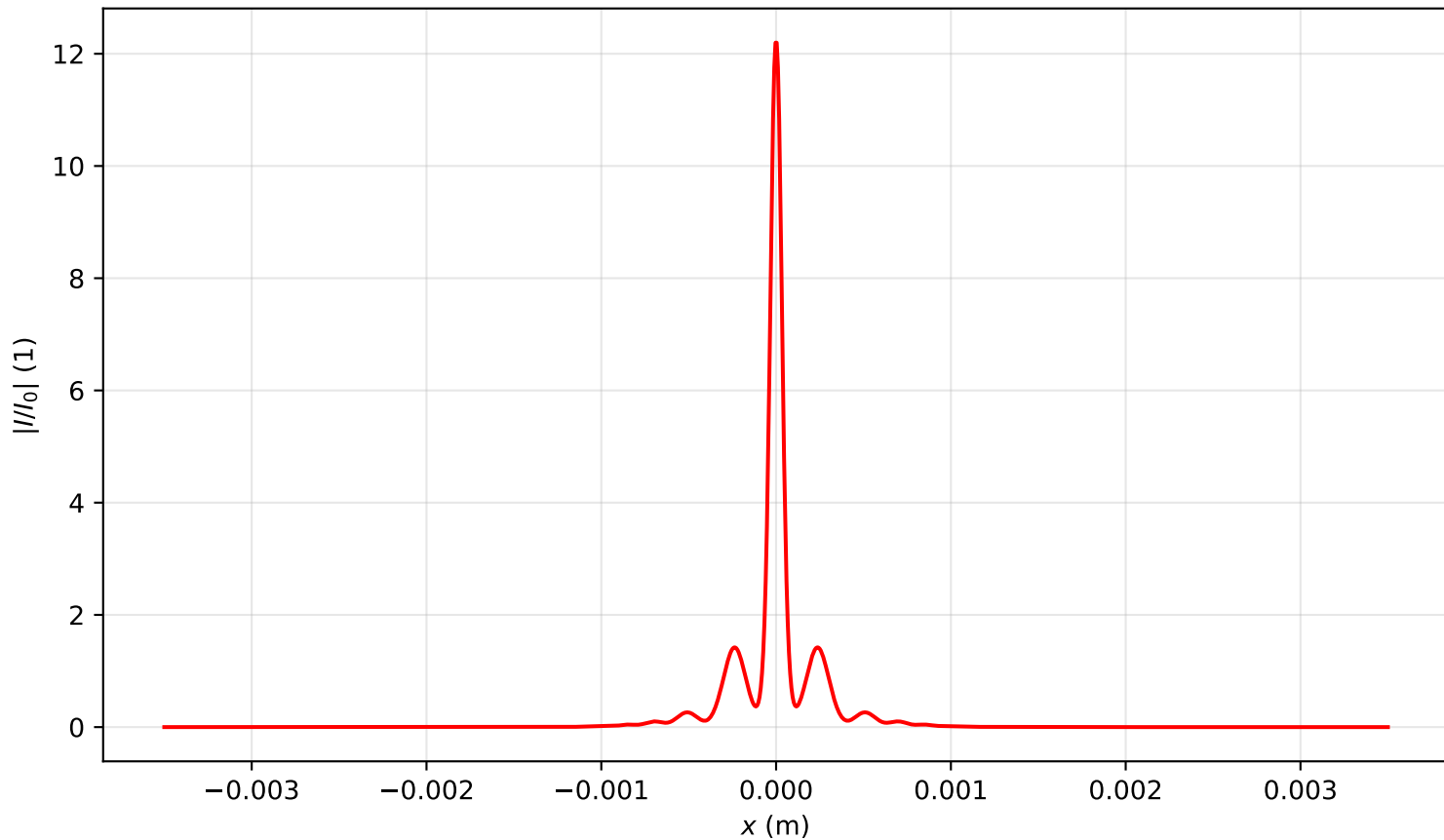
Intensity profile I(x, y = 0, z = 0.478)/I_0 , \text{Pin}=8.0\text{Pcr} , artificial time
